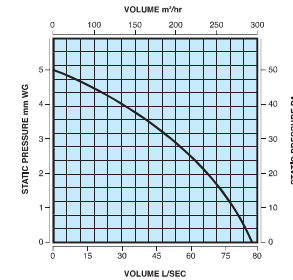
Performance Graph 150mm (6") series 278m 3 /hr, 77 litres per second
