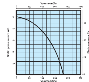
Performance Graph 300mm (12") series 1100m 3 /hr, 306 litres per second
