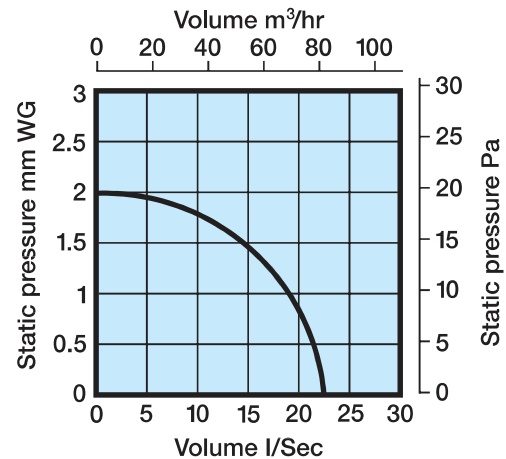
Performance Graph XF/WF100 Series 85m 3 /hr, 23 l/s
