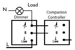
Fig 3. Alternative Wiring for 2 or 3-Way circuits
